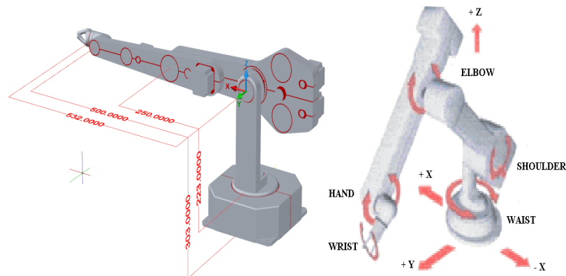
Figure 2: Bench Top R-12 Robot Arm Dimensions at JNEC, Aurangabad [2]
