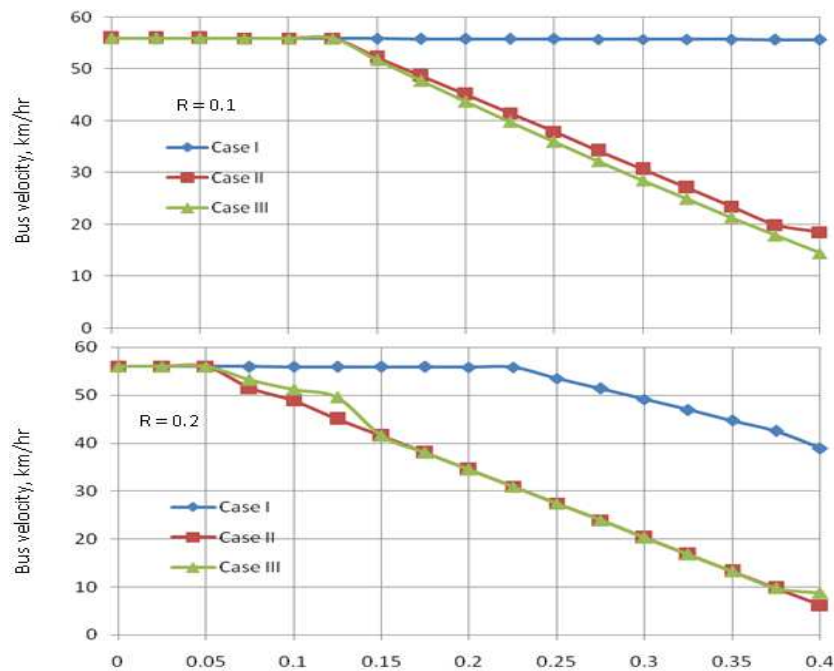
Figure 2: Profile of Velocity Density Profile of Buses
